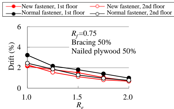
Figure 14: Maximum response drift of two-storied analysis model with double wood brace and nailed plywood under JMA Kobe wave
