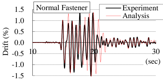
Figure 9: Time history of the case with normal brace fasteners under 50% of JMA Kobe wave
