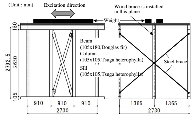
Figure 2: Wood frame for shake table test
