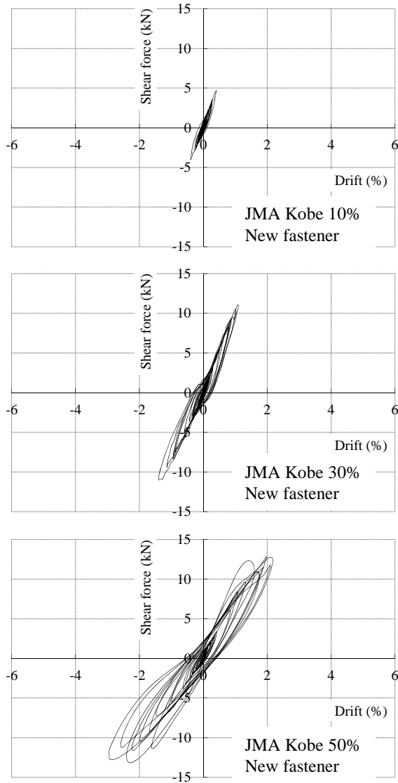
Figure 3: Shear force-drift relationship with double wood brace fastened by the new brace fasteners
