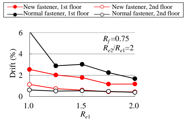
Figure 16: Maximum response drift of two-storied analysis model with twice R_e on second floor under JMA Kobe wave ( R_{e1} : R_e on first floor, R_{e2} : R_e on second floor)
