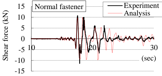
Figure 9: Time history of the case with normal brace fasteners under 50% of JMA Kobe wave
