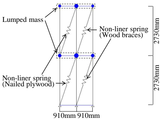
Figure 6: Analysis model of two-storied wooden house
