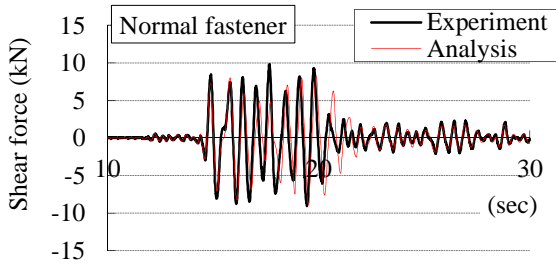
Figure 10: Time history of the case with normal brace fasteners under 30% of JMA Kobe wave
