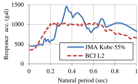
Figure 11: Response spectra ( h=5\% )
